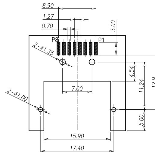
RECOMMENDED PCB LAYOUT (TOP VIEW) ALL TOLERANCES ARE \pm 0.05
