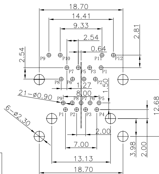
RECOMMENDED P.C.B LAYOUT TOP VIEW (COMPONENT SIDE)
